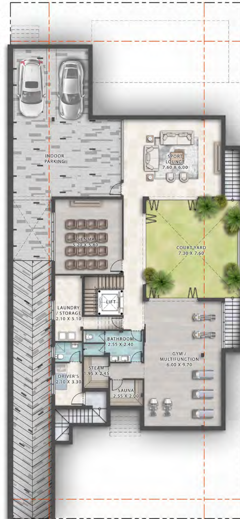
BASEMENT FLOOR
